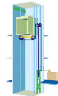
Single-cylinder side action type 4 : 2
