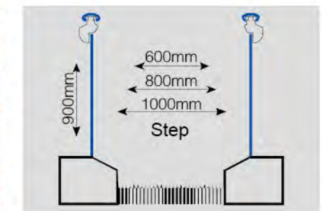
Balustrade Height (1000mm is standard specification)
