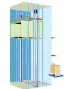
Double-cylinder side action 6-rail 2 : 1
